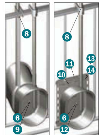
93.636/37
